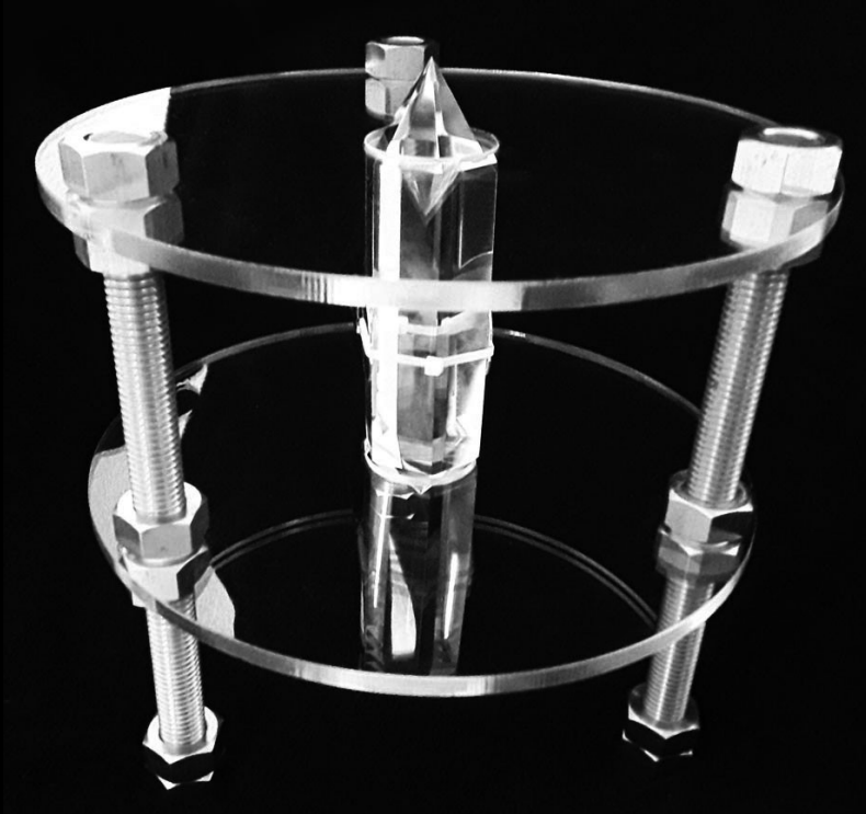
2 configurations to support the crystal with pure silver electrodes
